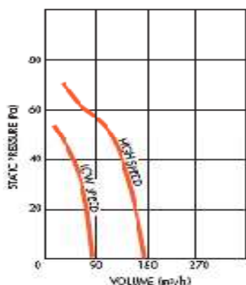
Centrif 170
